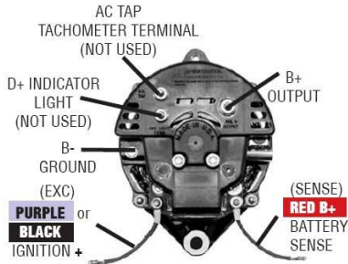
LATE MOTOROLA/PRESTOLITE STYLE FITS MERCURISER & OMC
