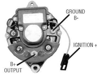
EARLY MOTOROLA STYLE FITS WESTERBEKE & OTHERS
