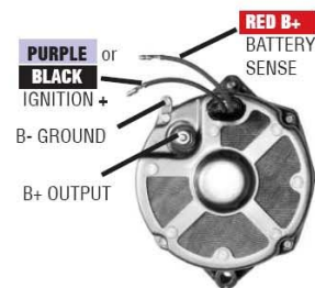
DELCO STYLE FITS MERCURISER & OMC
