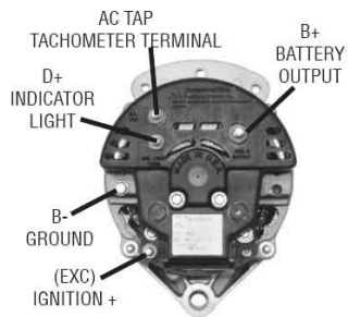
LATE MOTOROLA/PRESTOLITE STYLE FITS U.S. MARINE
