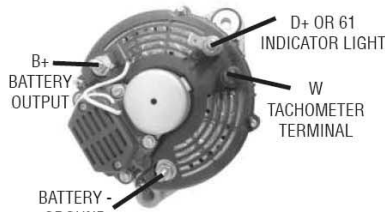
VALEO/PARIS RHONE FITS VOLVA PENTA
