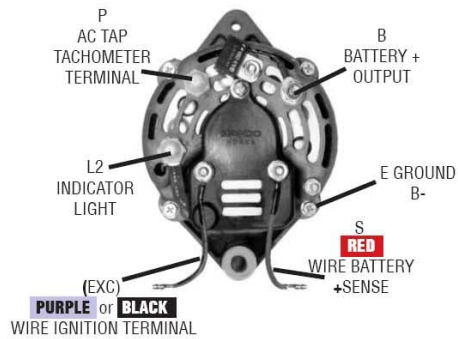
LATE MANDO STYLE FITS MERCURISER & OTHERS
