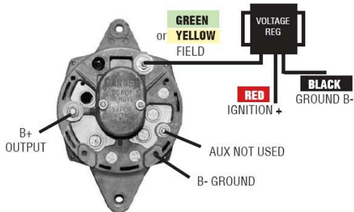
EARLY PRESTOLITE STYLE FITS OMC
